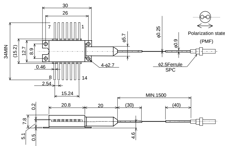
Package outline(Unit:mm) Type:AF4A1204A75L
